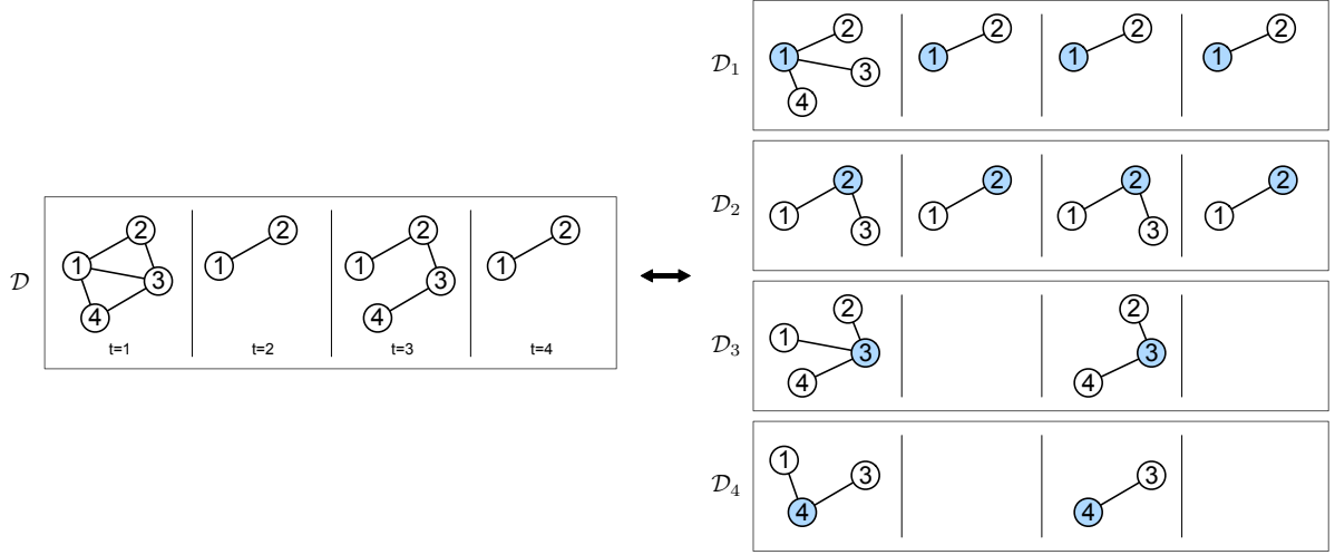
Figure 2: A global dynamic encounter graph \mathcal{D} and its intrinsic dynamic encounter graphs. \mathcal{D}_v denotes the intrinsic dynamic encounter graph for node v .
